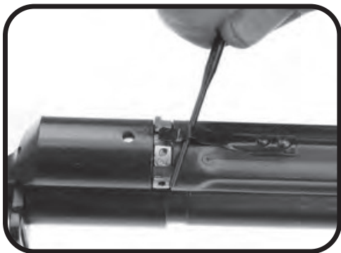
Picture #23-Lifting the spring securing pin
