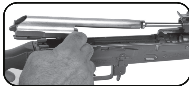
Picture #14 Remove bolt and carrier
