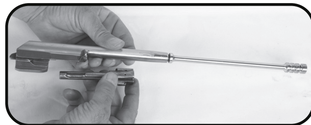
Picture #15 Separate bolt from carrier
